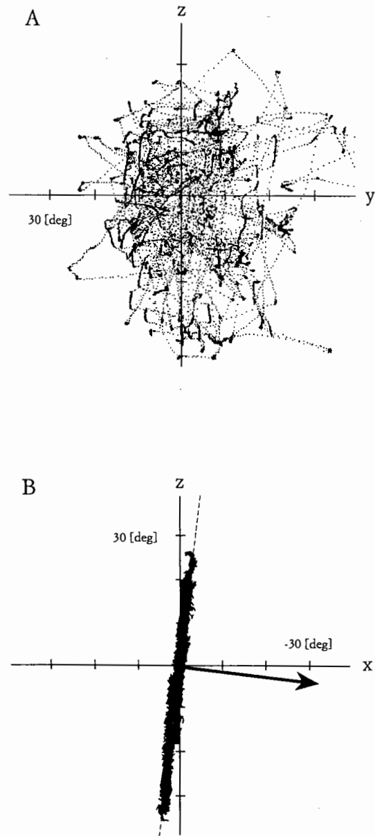
FIGURE 2. Rotation vectors of a recording of 90 sec of spontaneous eye movements in the light, while the monkey was in the upright position. (A) Frontal view of the eye rotation vectors, with the z-components plotted against the y-components. Points on the z-axis correspond to eye positions reached by a rotation from the reference position about the z-axis, i.e. horizontal eye positions, points on the y-axis correspond to vertical eye positions. (B) Side view of the same data, with the z-components vs the x-components (torsional eye positions). All rotation vectors are approximately confined to a plane, which is indicated by the thin, dashed line. The arrow shows the orientation of the plane. The SD of the data points from this plane is 0.6°.
