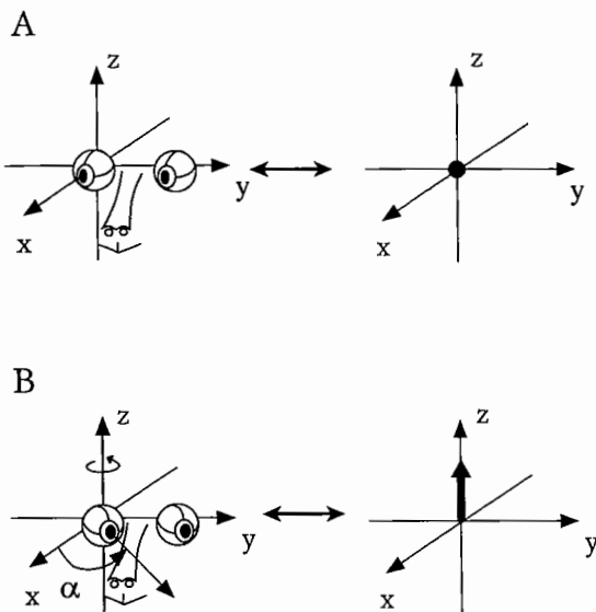
FIGURE 1. Every eye position is characterized by one rotation vector: (A) the reference position corresponds to the origin of the rotation-vector space (zero rotation vector). (B) Every other position corresponds to one rotation from the reference position to the current eye position. The direction of the respective rotation vector is given by the axis of this rotation, and its length by \tan(\alpha/2) , with \alpha the angle of the rotation.
